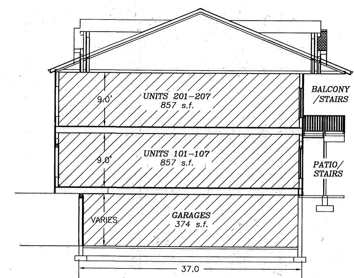
CROSS SECTION SCALE: 1"=10'
