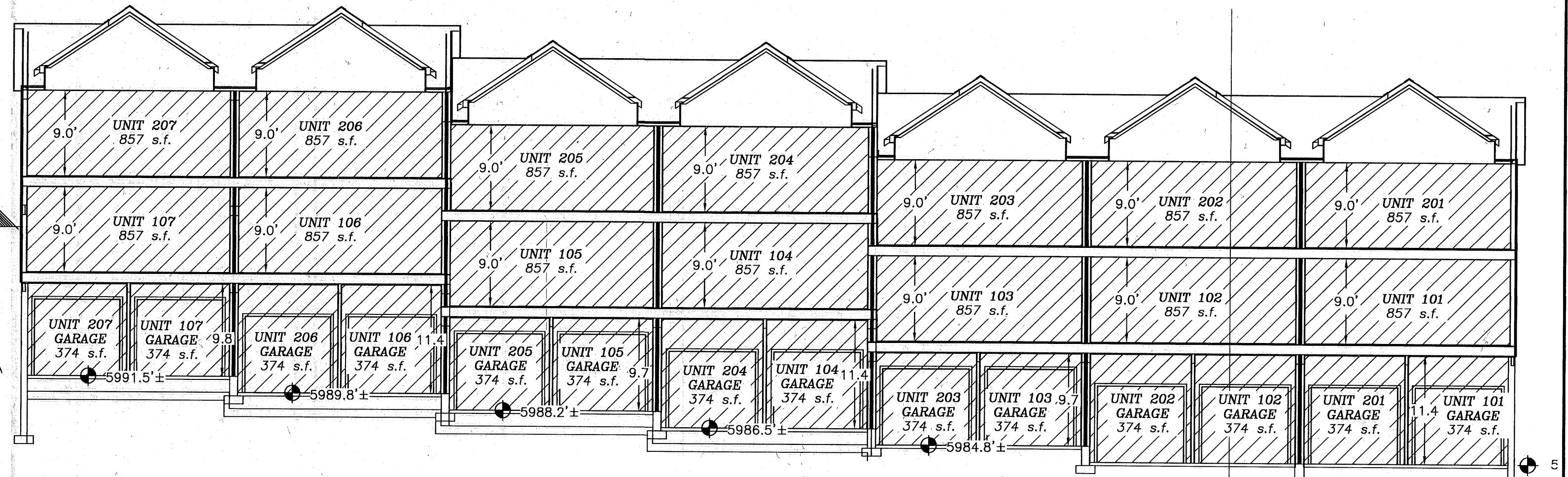
CROSS SECTION SCALE: 1"=10'
