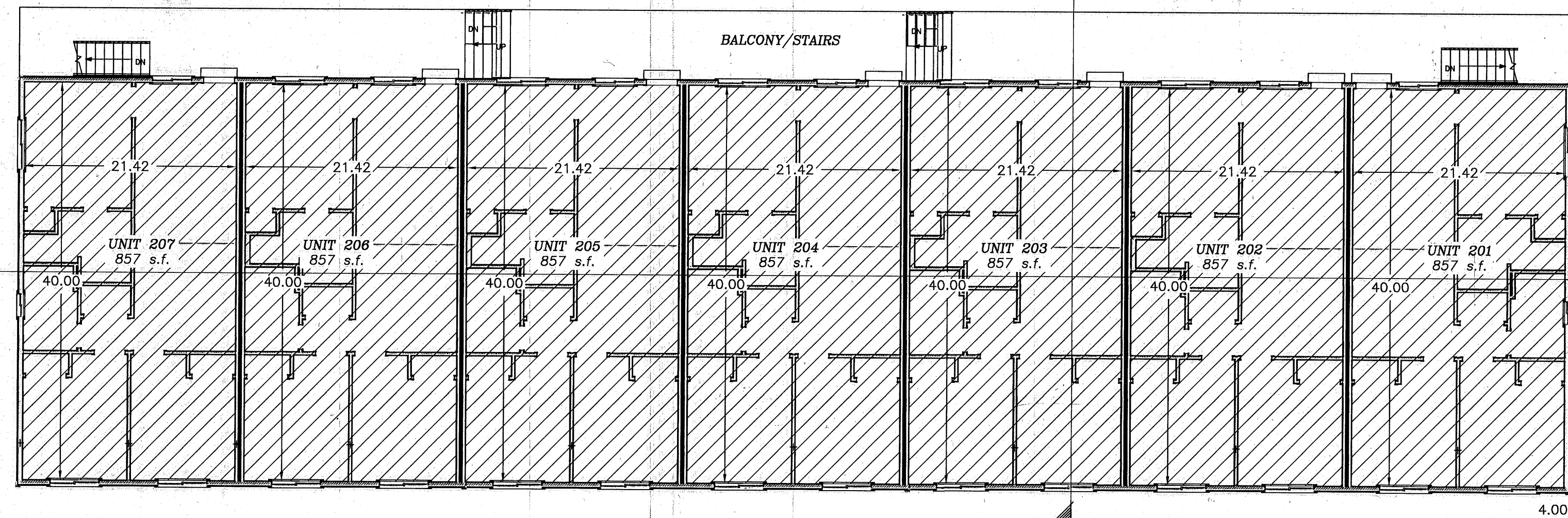
3rd FLOOR LEVEL (CONDO B) SCALE: 1"=10'
